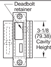
Model 662 RH Strike For latch & deadbolt combination locksets
