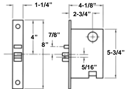
Mortise Lock Dimensions
